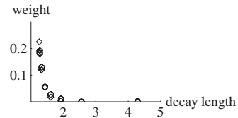
FIG. 4. Weights of the wave function passing through the junction sketched in Fig. 2 on evanescent waves of different decay lengths. The width of the junction is 16 unit cells and there are 30 evanescent waves. The decay length is in units of the lattice spacing in the direction parallel to the edges ( \sqrt{3} \times a , where a is the C-C bond). Diamonds show waves symmetric around the junction and hexagons show antisymmetric waves (note that the waves studied here decay as function of the distance to the junction, not to the edges of the ribbon).
