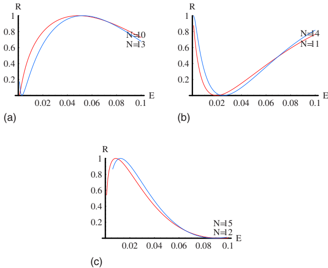
FIG. 3. (Color online). Reflection at a 60^\circ junction like the one sketched in Fig. 2 for different junction widths. N gives the number of unit cells across the junction. The width of each ribbon that makes up the junction is 3/2aN where a is the length of the C-C bond. The energy is in units of the nearest-neighbor hopping.
