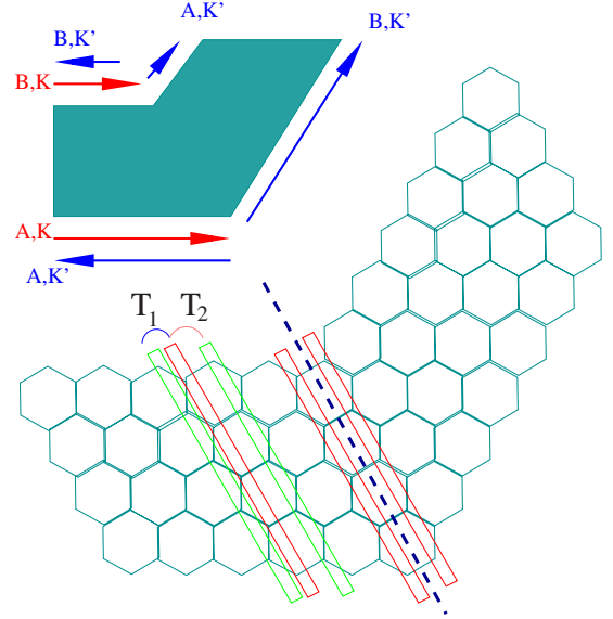
FIG. 2. (Color online) Sketch of the 60^\circ junction analyzed in the text. Top left: an incoming wave from the left, built up from eigenstates in the vicinity of the K valley, has to be either transmitted or reflected as a superposition of states from the K' valley. Bottom: Scheme used to analyze the transmission in the honeycomb lattice. The junction has a reflection symmetry around its center, shown as dashed line. On each side, the nearest-neighbor hopping problem can be written as a sum of coupling between nearest-neighbor transverse stripes. See text for details.
